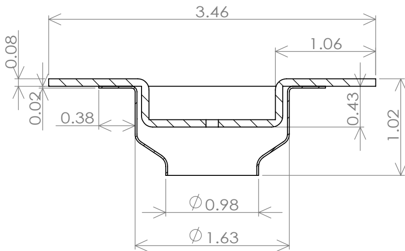
A cross section A-A
