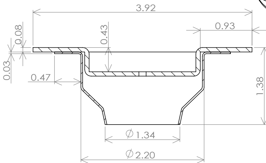
A cross section A-A
